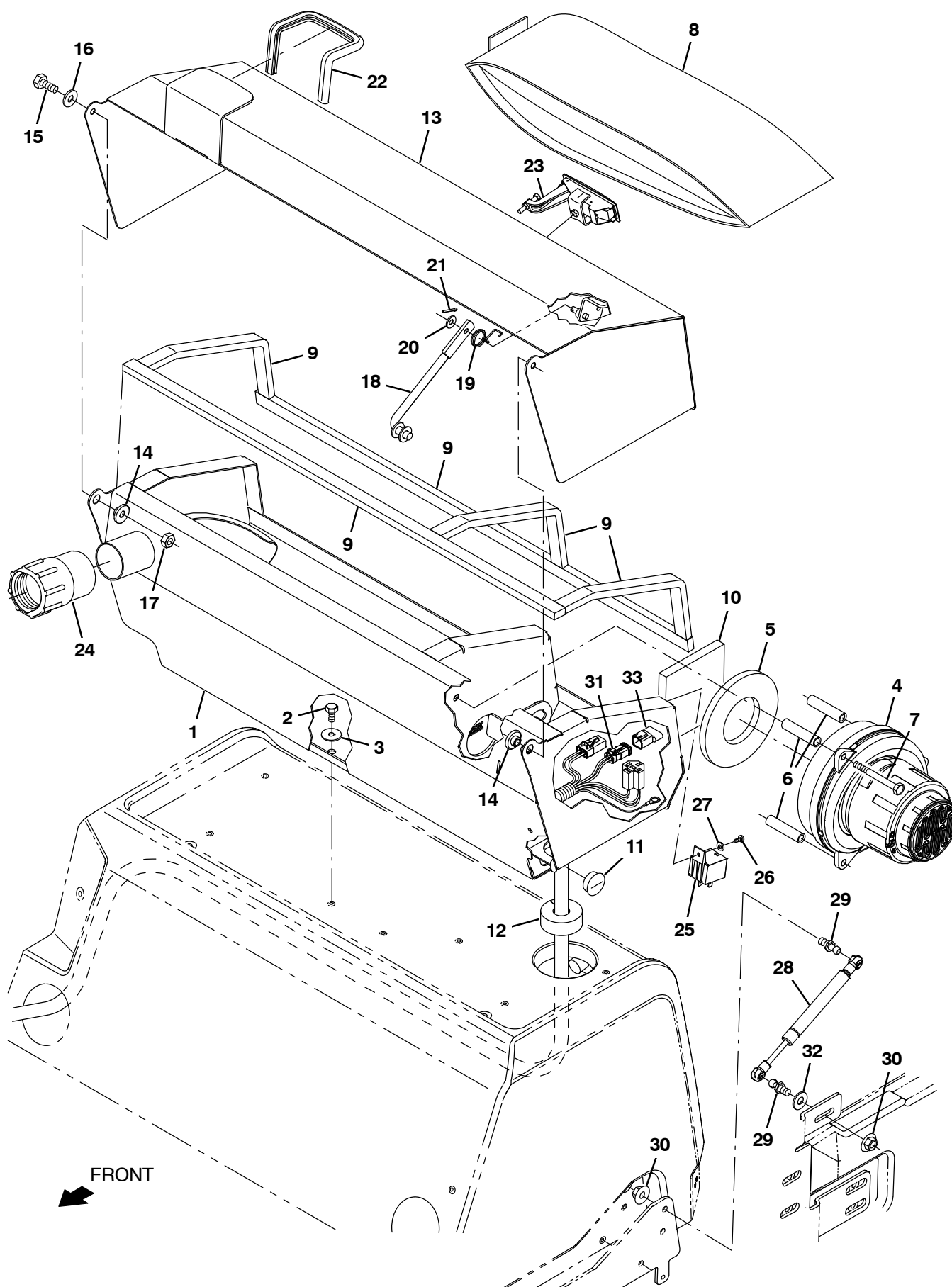
Fig. 3 – Vacuum Wand Box and Fan Group
