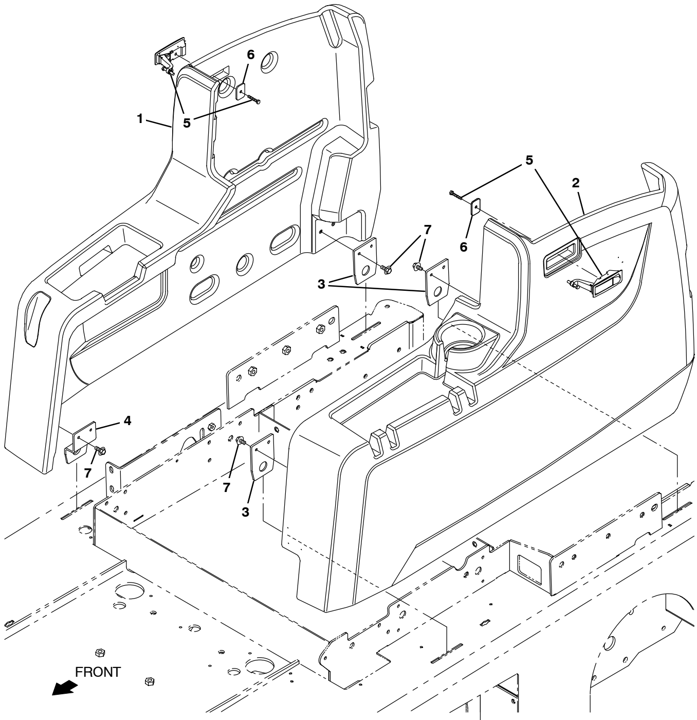
Fig. 3 – Shrouds Group
