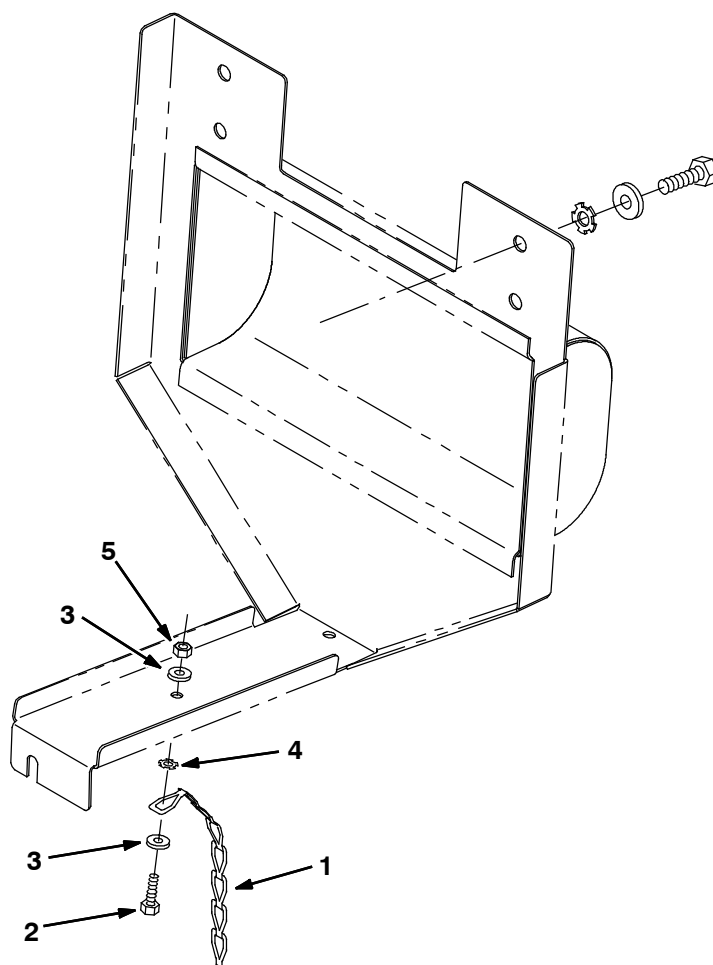
Fig. 18 - Steel Static Chain Kit
