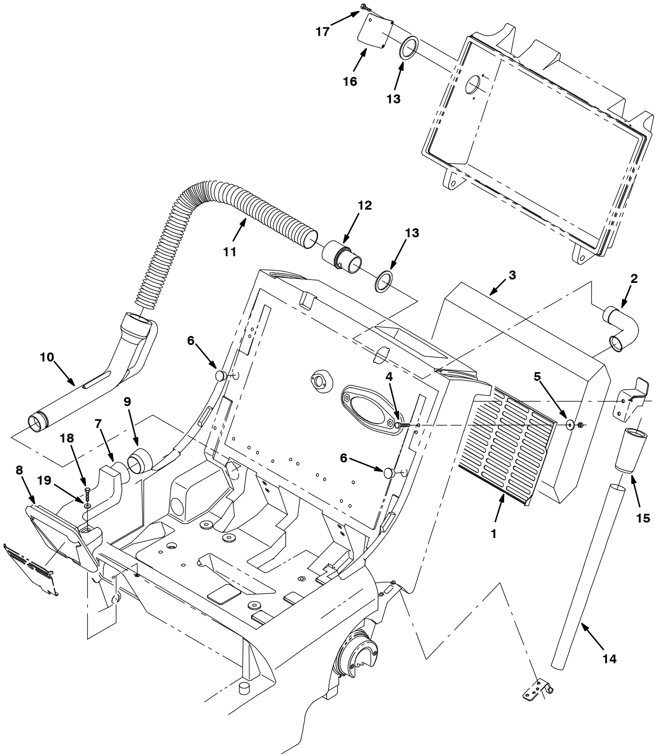
Fig. 5 - High Flow To Standard Bag Kit
