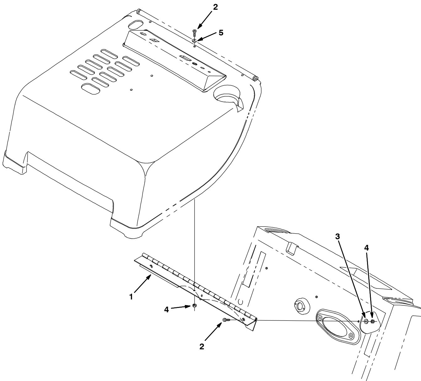
Fig. 20 - Hinge Repair Kit
